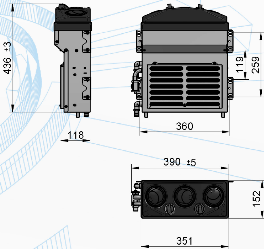
HVAC Unit
